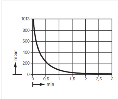
Pump down time for 10 l receiver
