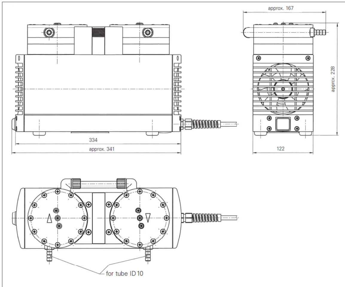
Dimensions (mm)
